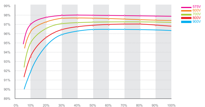
Growatt 9000UE efficiency
